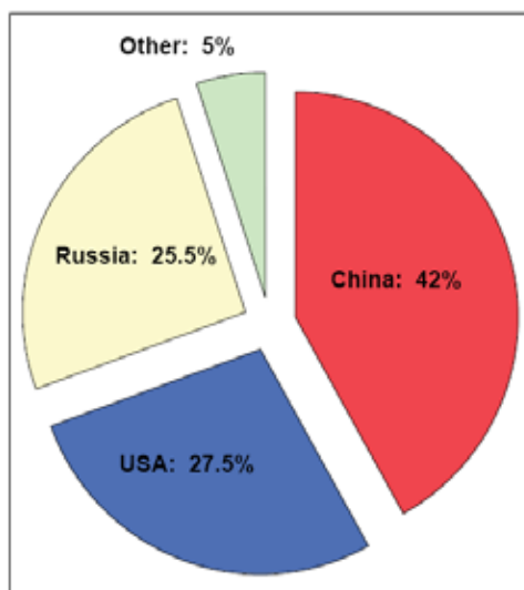
Figure 2. The People's Republic of China was responsible for nearly half of all known satellite breakup debris in orbit as of 1 January 2008. The
