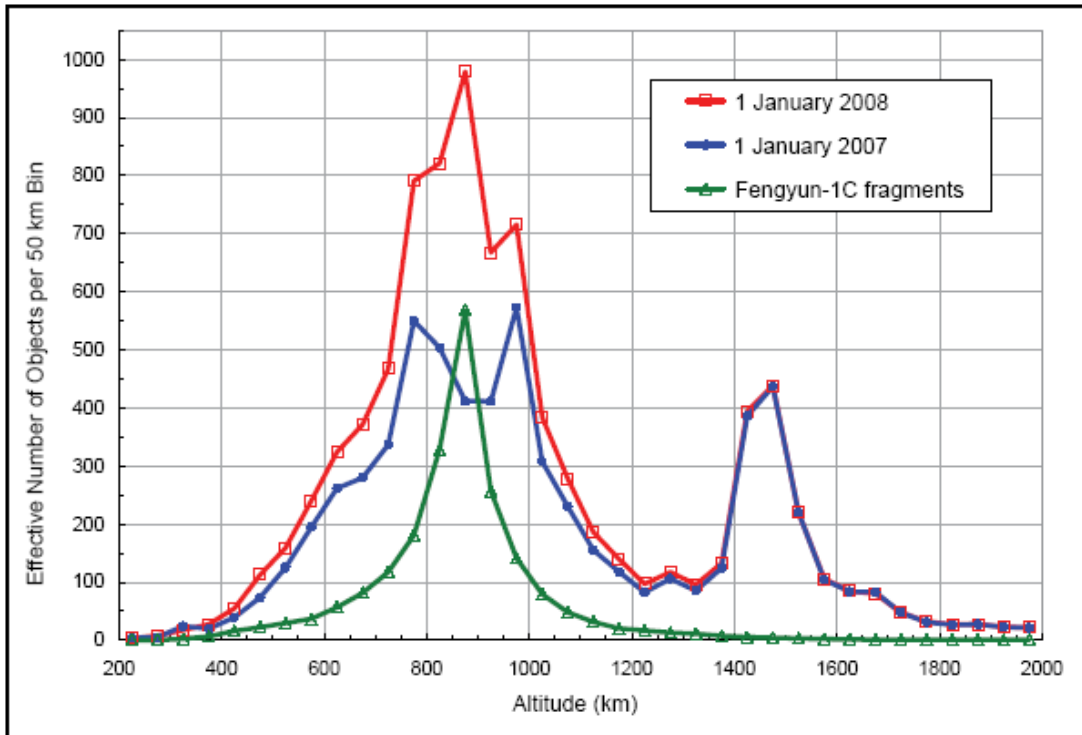
Figure 1. Distributions of the catalog populations in the low Earth orbit region in January 2007 (blue), January 2008 (red), and the officially
